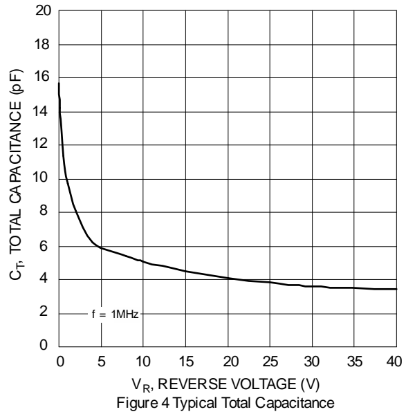
Figure 4 Typical Total Capacitance
